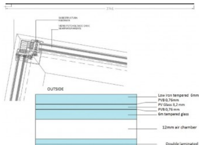
Details of glass configuration and installation on the supporting structure © Onyx Solar
